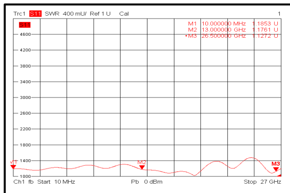
VSWR @+25°C
