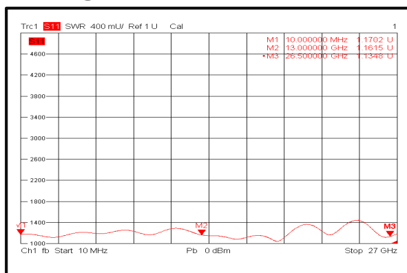
VSWR @+85°C
