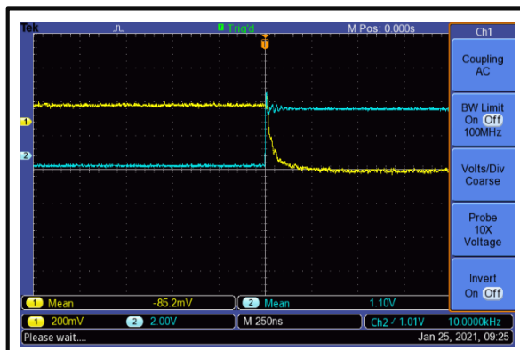
Fall Time
